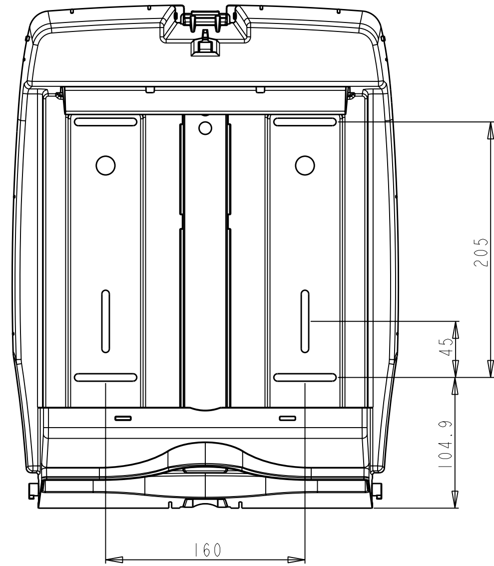
Drill pattern
